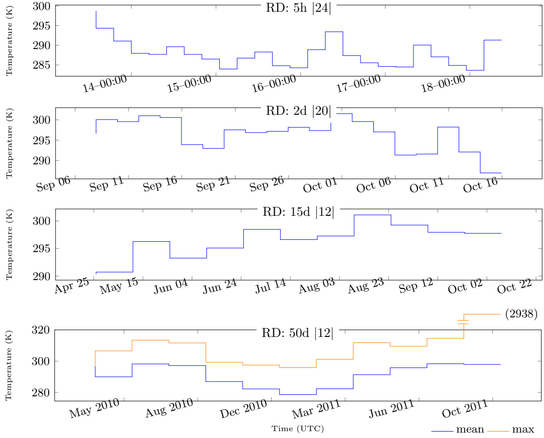
Figure 6: Resolution discs' time series in a MTSDDB
